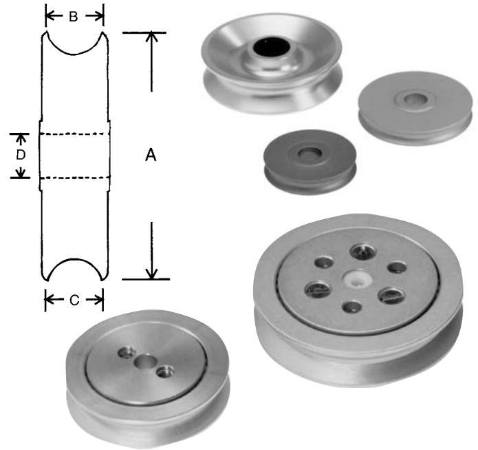
Aluminium sheave
