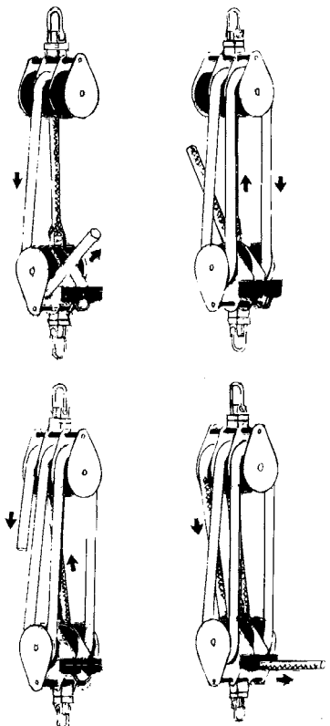
Method of reeving triple purchase with blocks having central becket and exit from centre sheave
